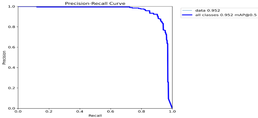
Fig. 5. The precision–recall curve Source: Own study
