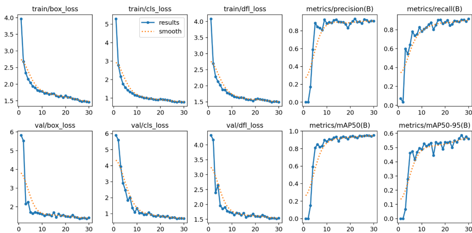
Fig. 2. Learning curves and validation metrics (YOLOv8)
