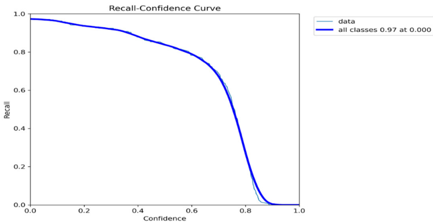
Fig. 6. The recall–confidence curve Source: Own study
