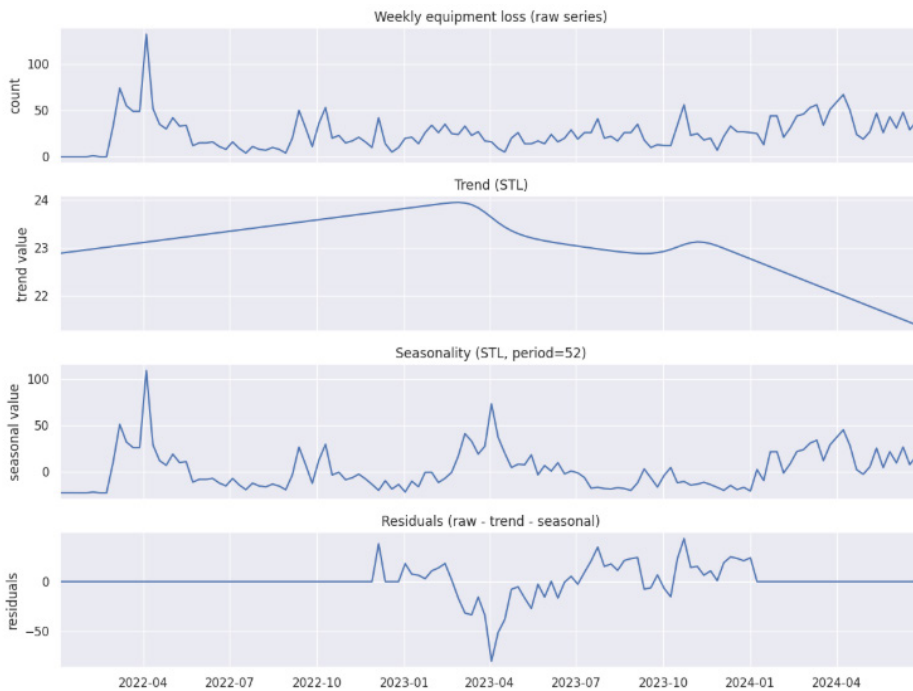
Fig. 8. STL decomposition of the weekly series
