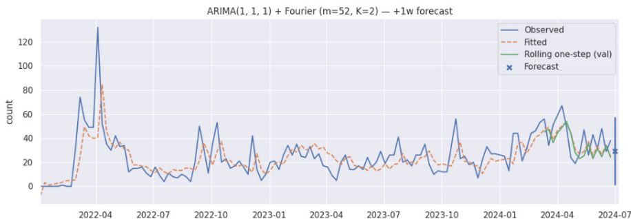
Fig. 12. ARIMA(1,1,1) + Fourier (m = 52, K = 2) - +1w forecast
