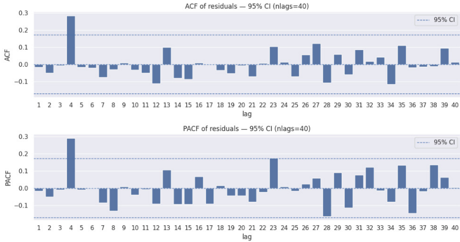
Fig. 13. ACF/PACF of ARIMAX residuals
