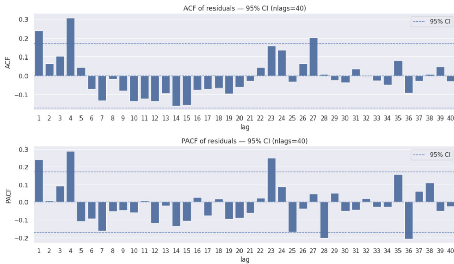
Fig. 11. Residual ACF/PACF for SARIMA(1,1,1)(0,1,1)[52]
