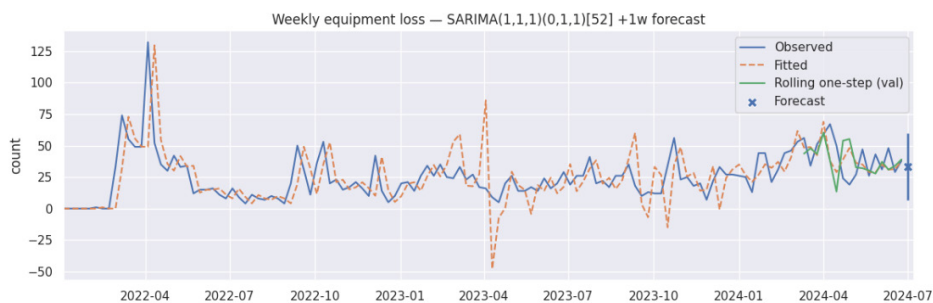
Fig. 10. Weekly equipment losses – SARIMA(1,1,1)(0,1,1)[52] with +1-week forecast (16-week rolling validation)
