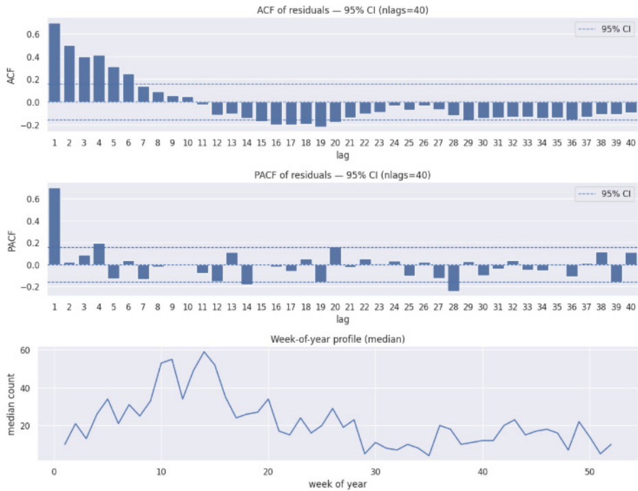
Fig. 9. Residual autocorrelation (ACF) and partial autocorrelation (PACF)
