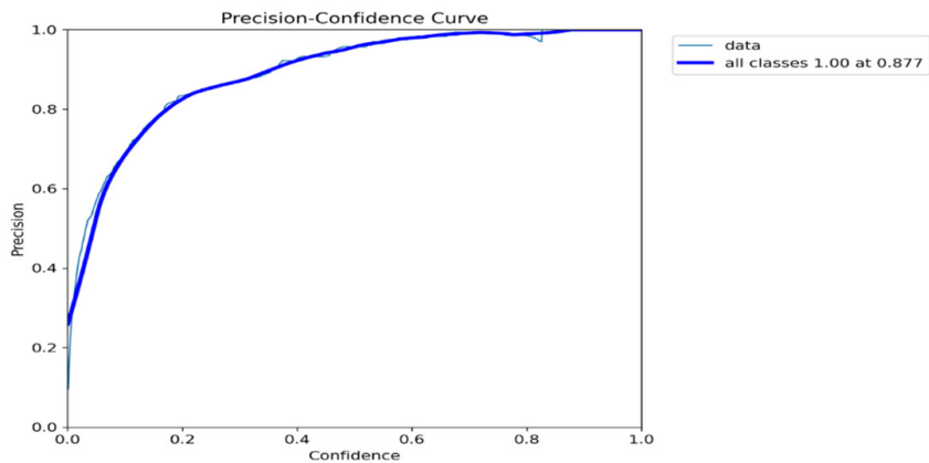
Fig. 4. The precision–confidence curve
